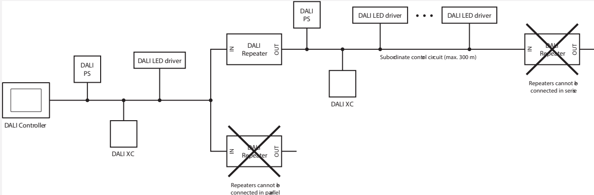
3.3 Multi-Master application
