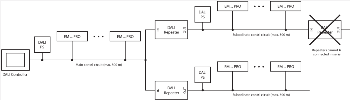
Single-Master application
